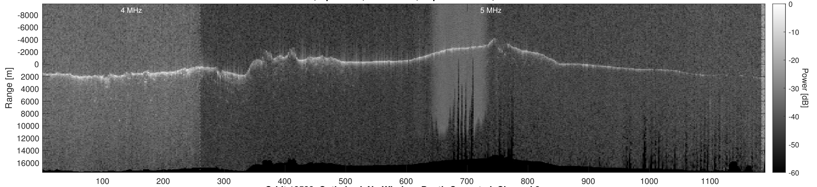
Orbit 12533, Optimized, No Window, Depth-Corrected, Channel 2
