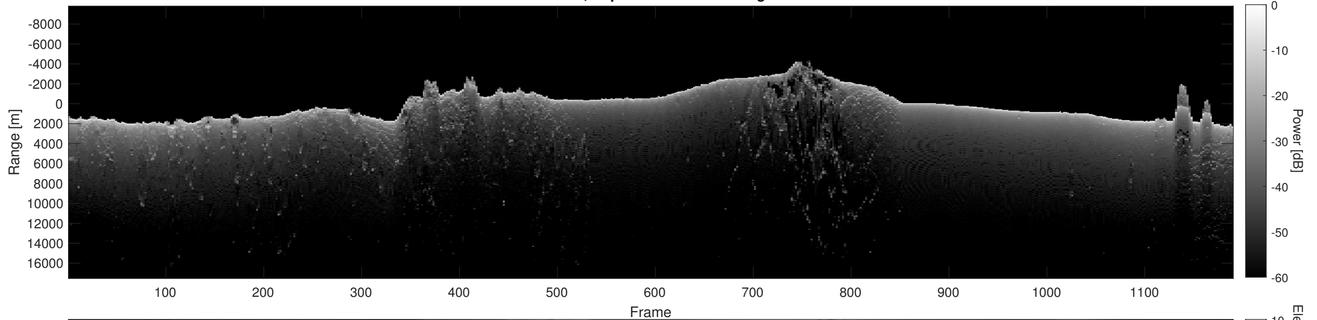
Orbit 12533, Depth-Corrected Cluttergram
