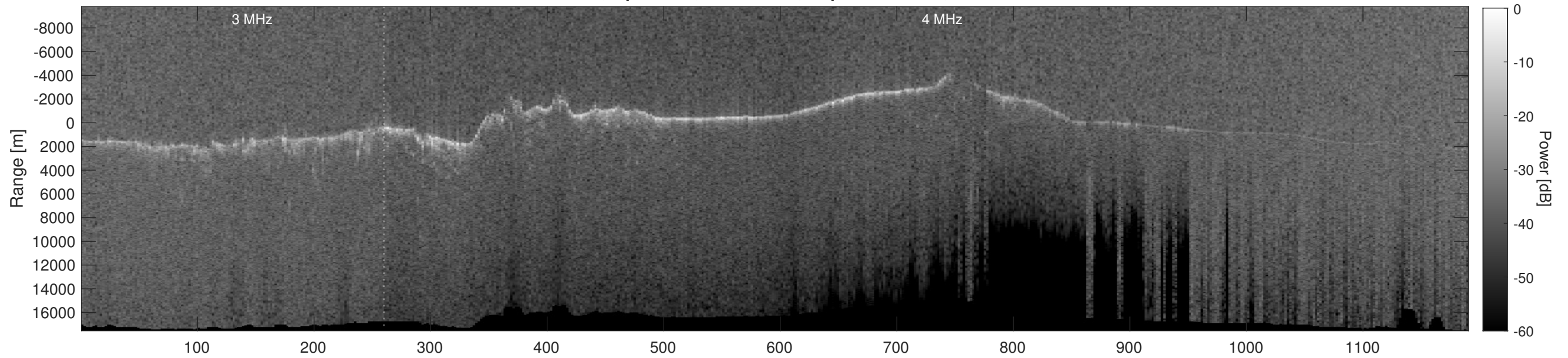
Orbit 12533, Depth-Corrected Cluttergram
