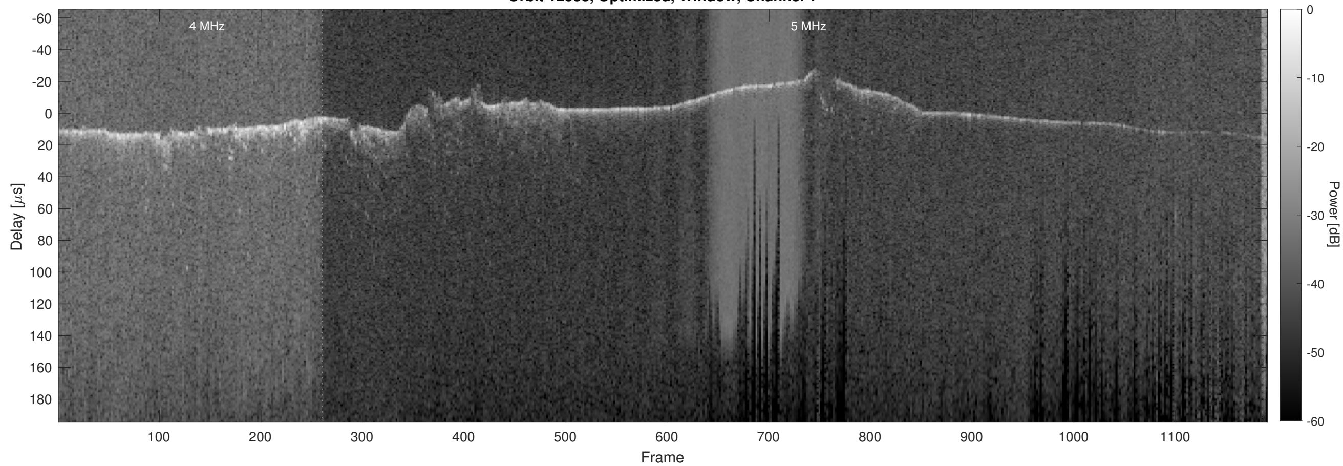
Orbit 12533, Optimized, Window, Channel 2
