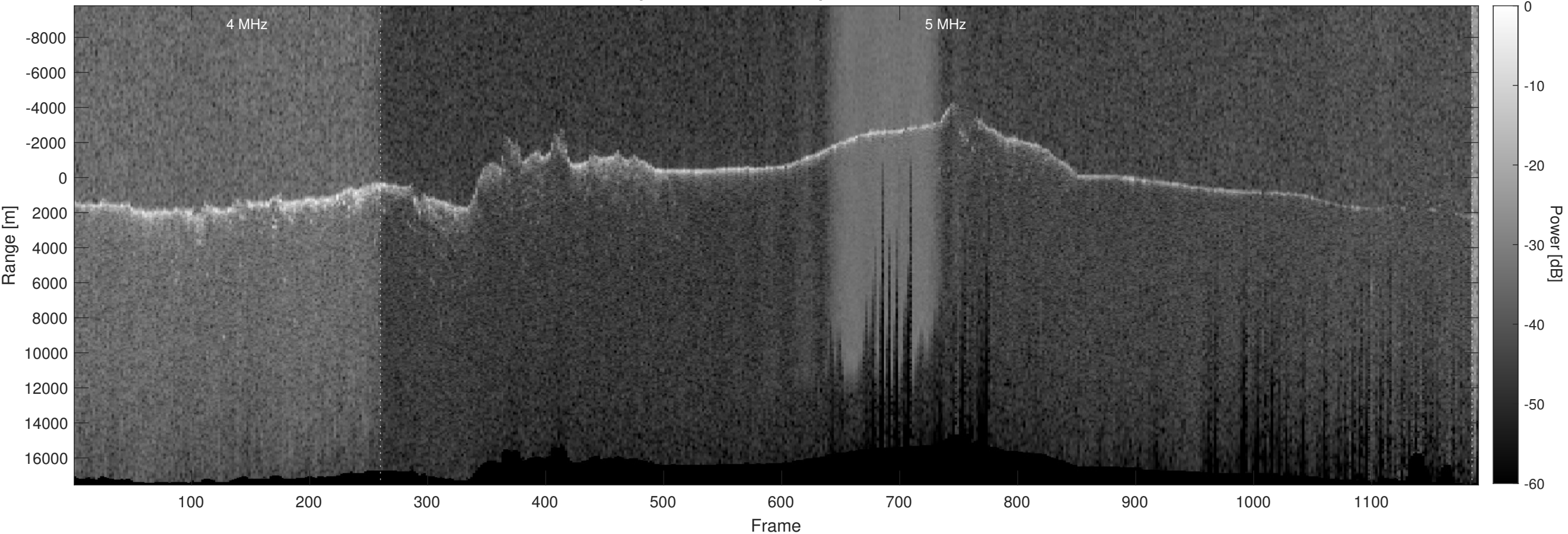
Orbit 12533, Optimized, Window, Depth-Corrected, Channel 2
