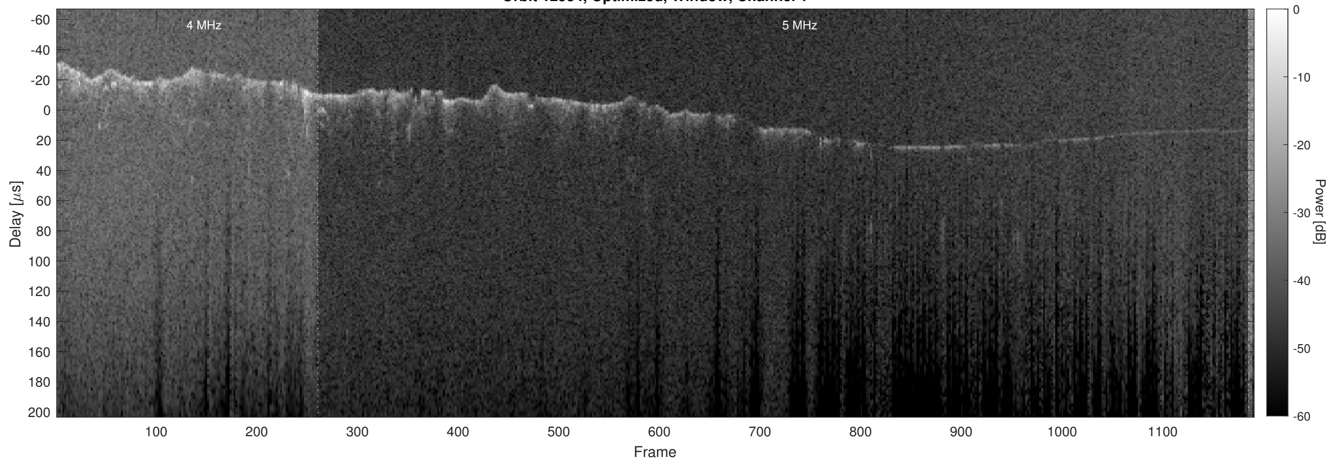
Orbit 12534, Optimized, Window, Channel 2
