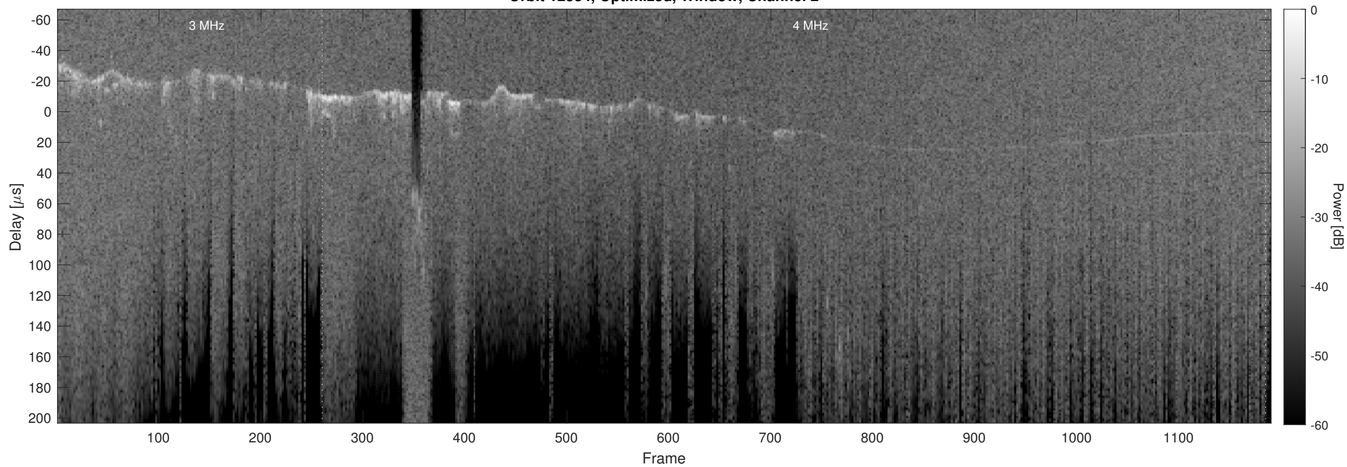
Orbit 12534, Optimized, Window, Channel 2
