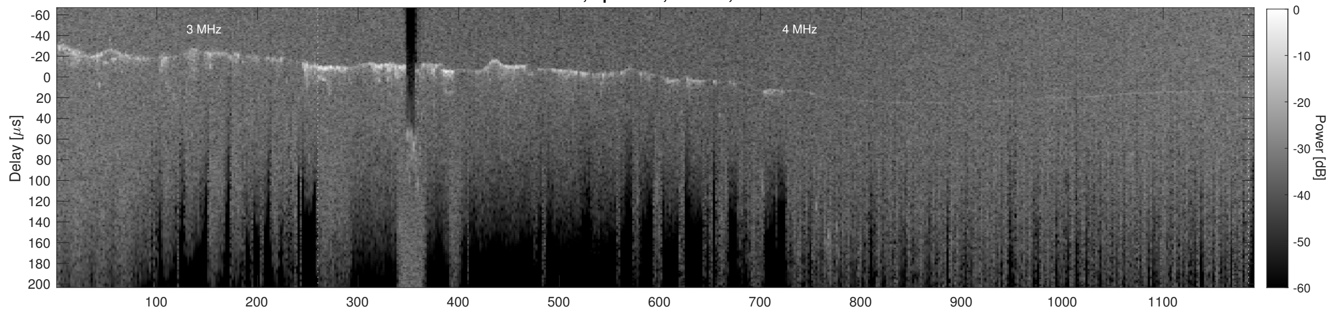
Orbit 12534, Cluttergram
