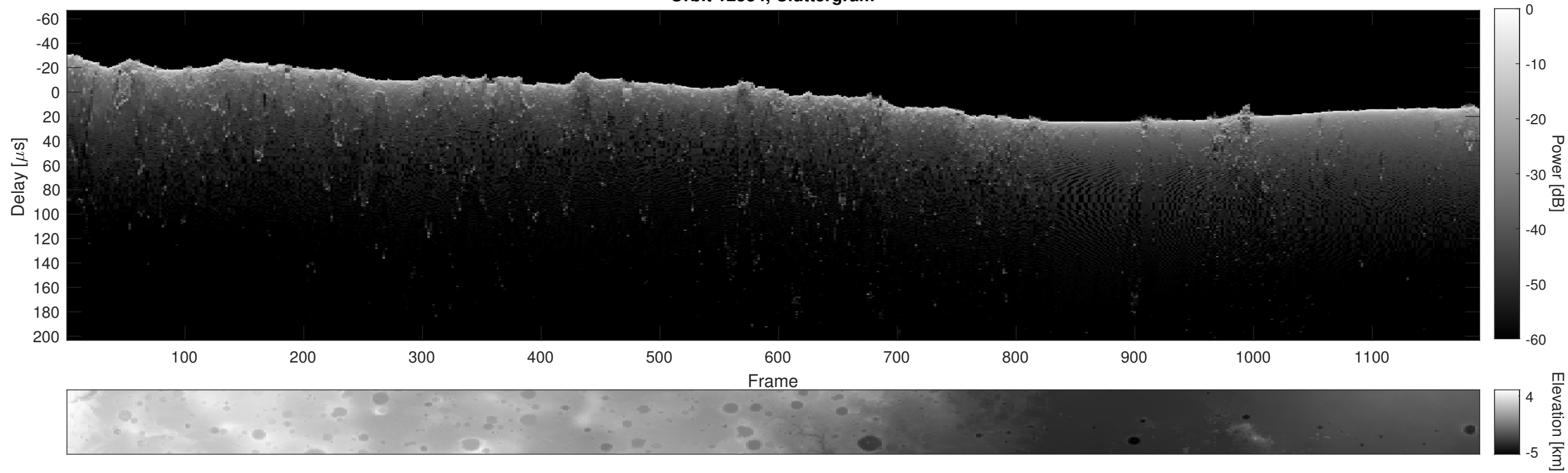
Orbit 12534, Cluttergram
