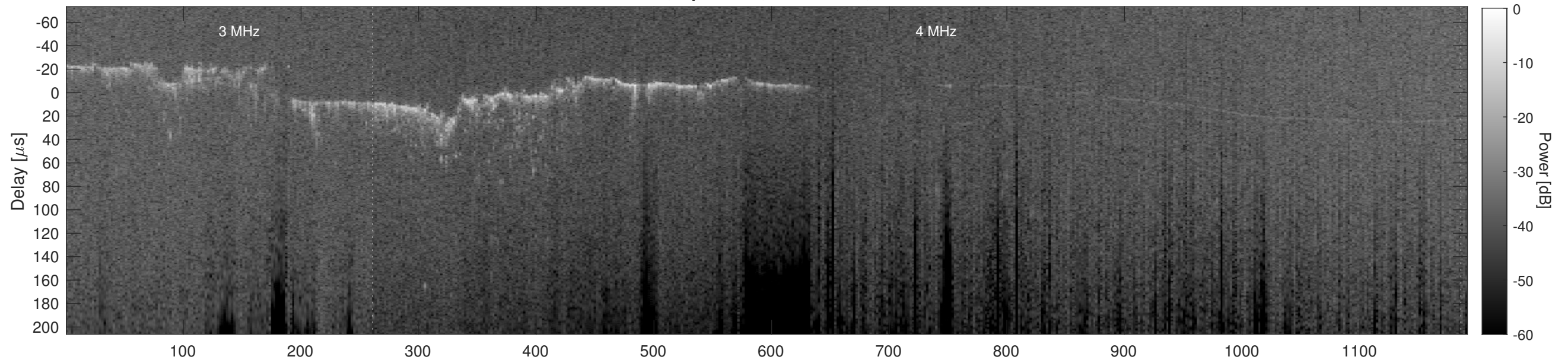
Orbit 12536, Cluttergram
