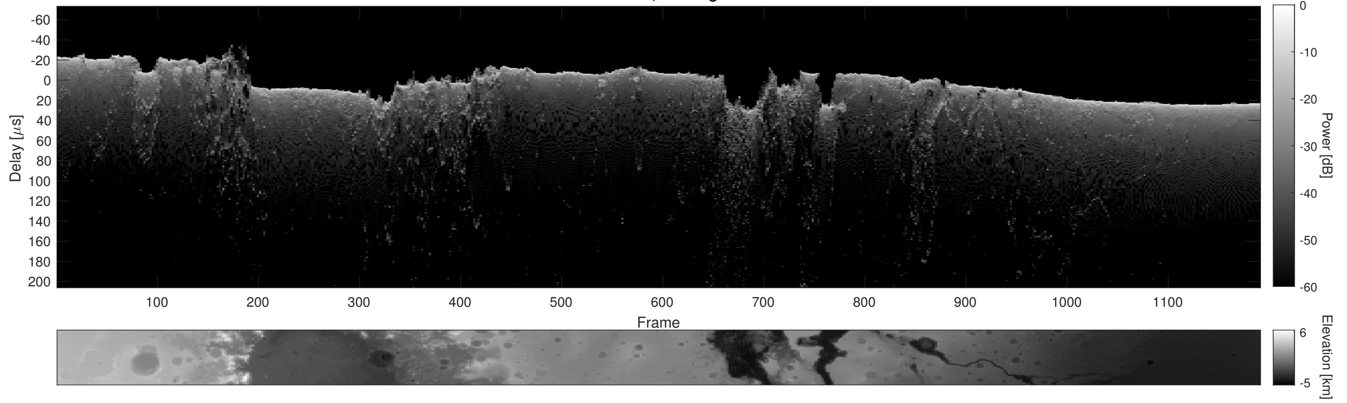
Orbit 12536, Cluttergram
