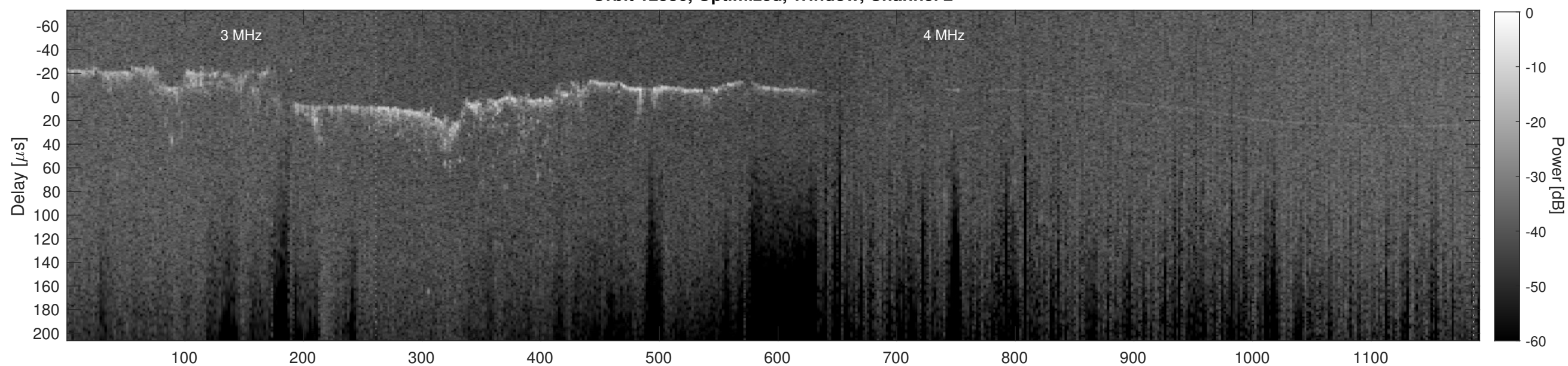
Orbit 12536, Cluttergram
