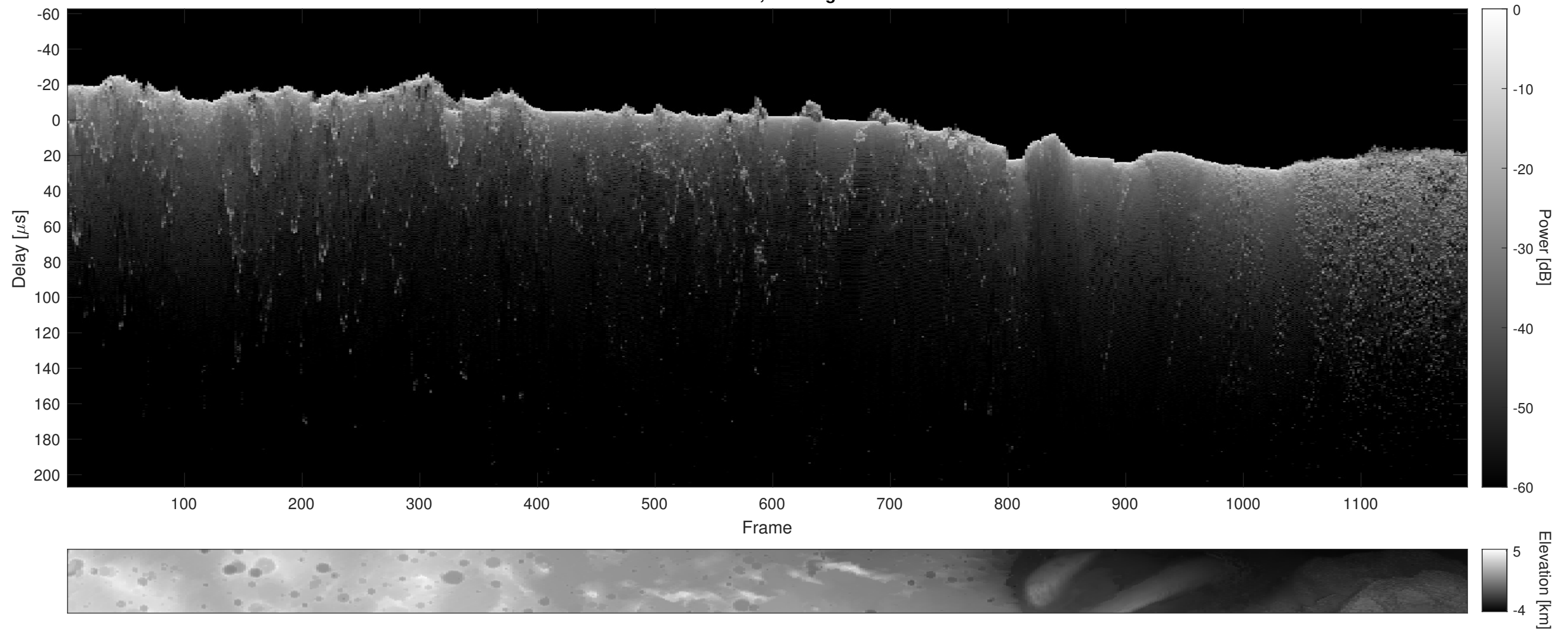
Orbit 12537, Cluttergram
