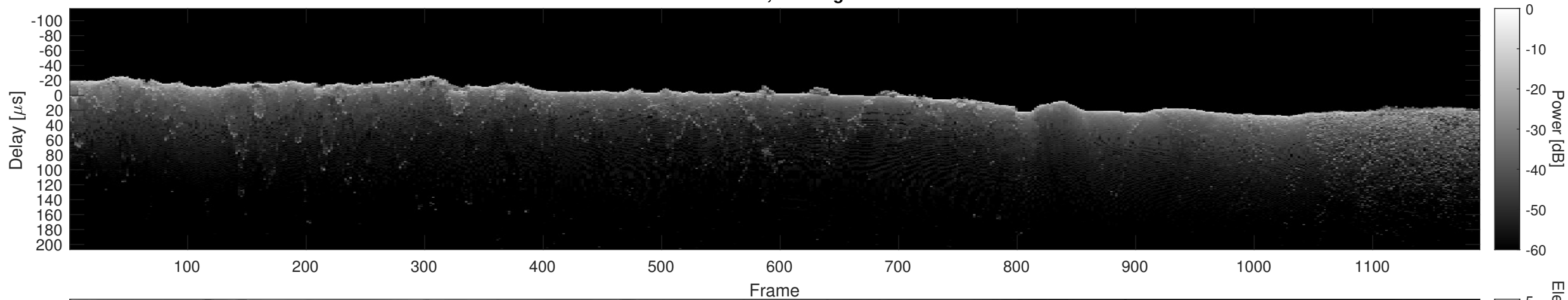
Orbit 12537, Cluttergram
