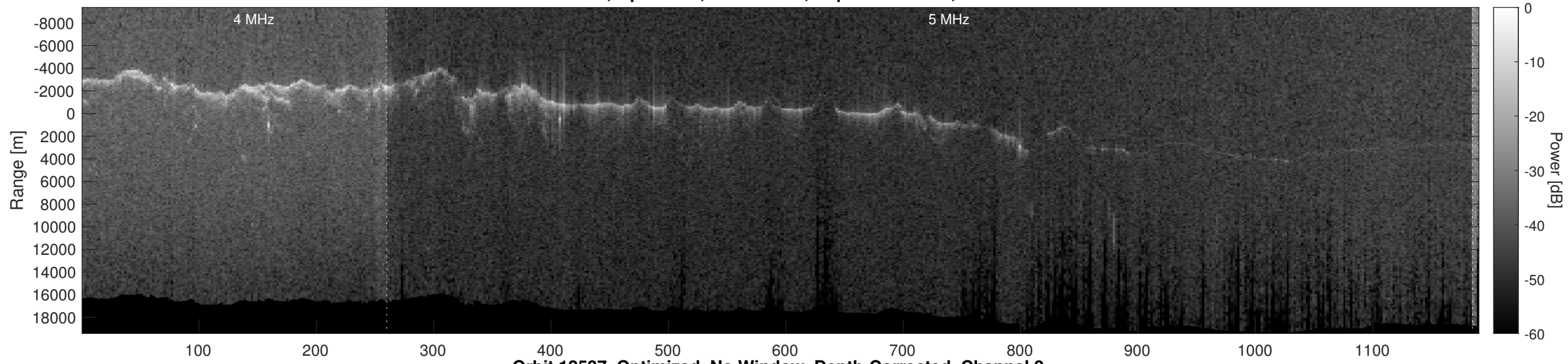
Orbit 12537, Optimized, No Window, Depth-Corrected, Channel 2
