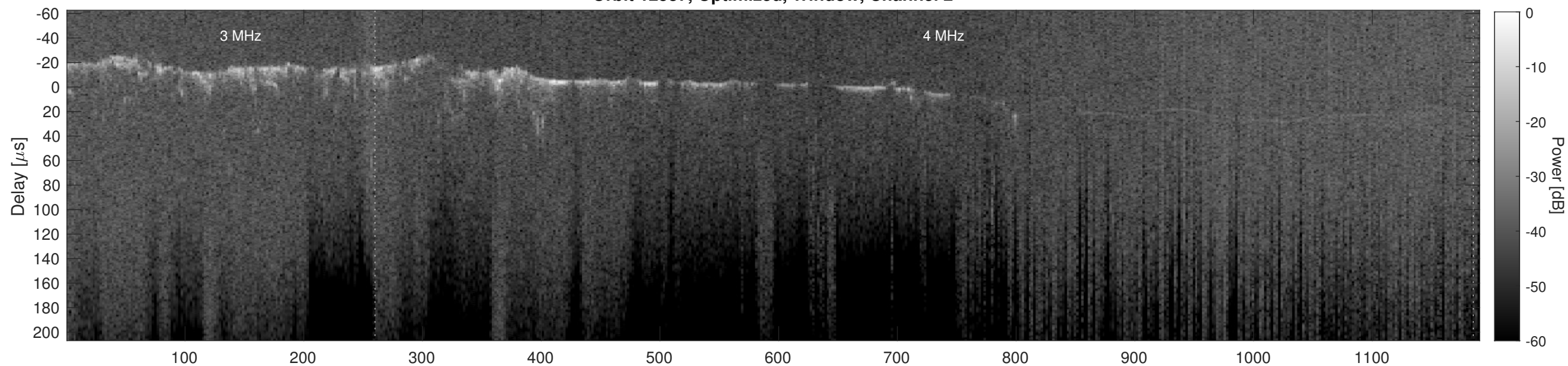
Orbit 12537, Cluttergram
