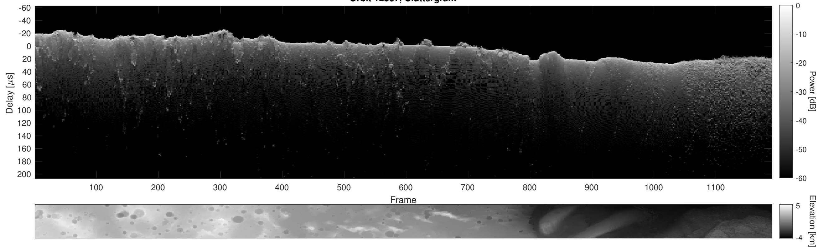
Orbit 12537, Cluttergram
