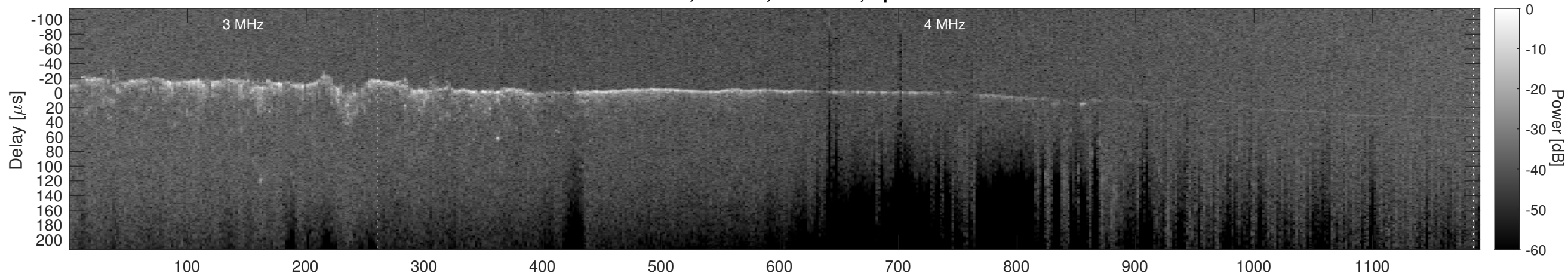
Orbit 12538, Cluttergram
