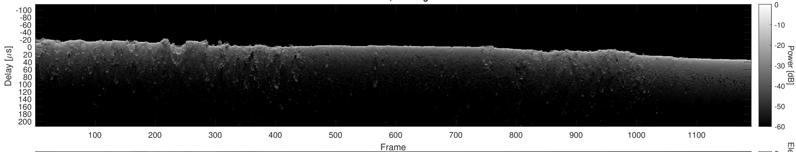
Orbit 12538, Cluttergram
