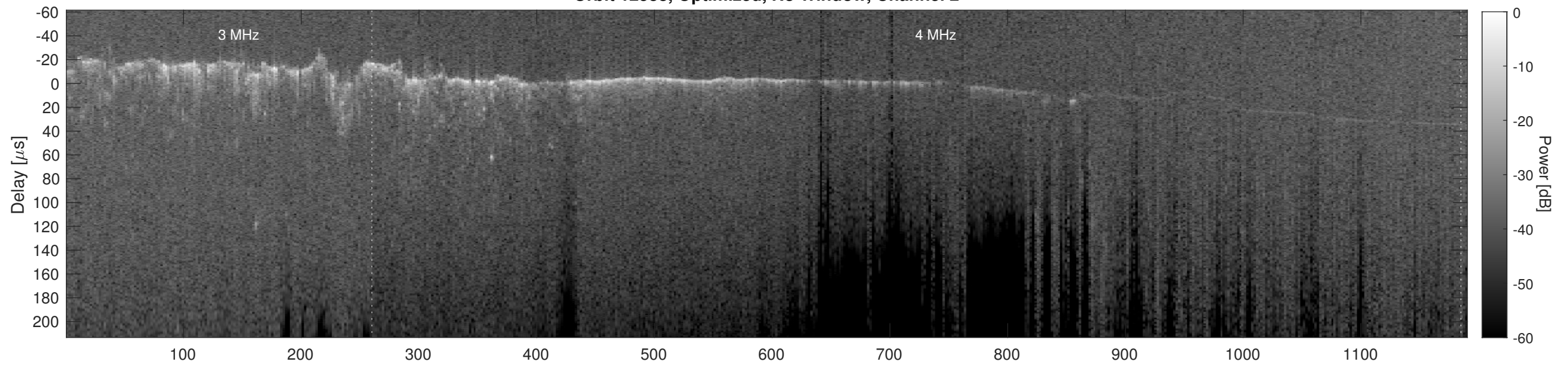
Orbit 12538, Cluttergram
