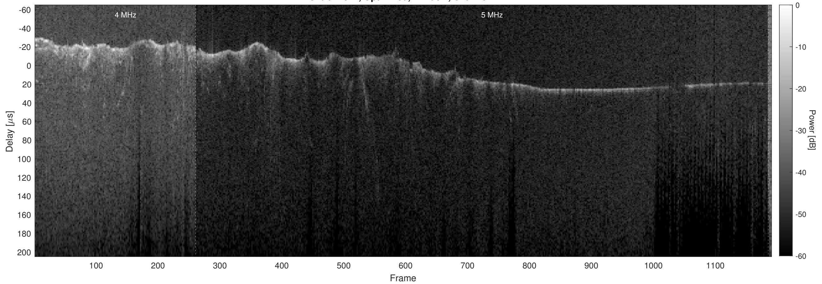
Orbit 12541, Optimized, Window, Channel 2
