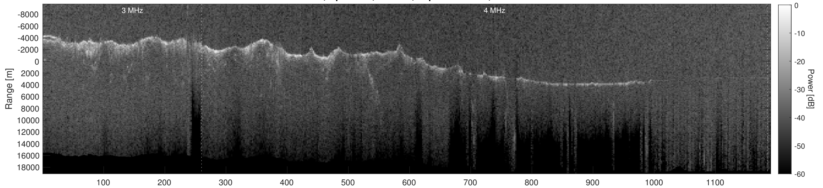
Orbit 12541, Depth-Corrected Cluttergram
