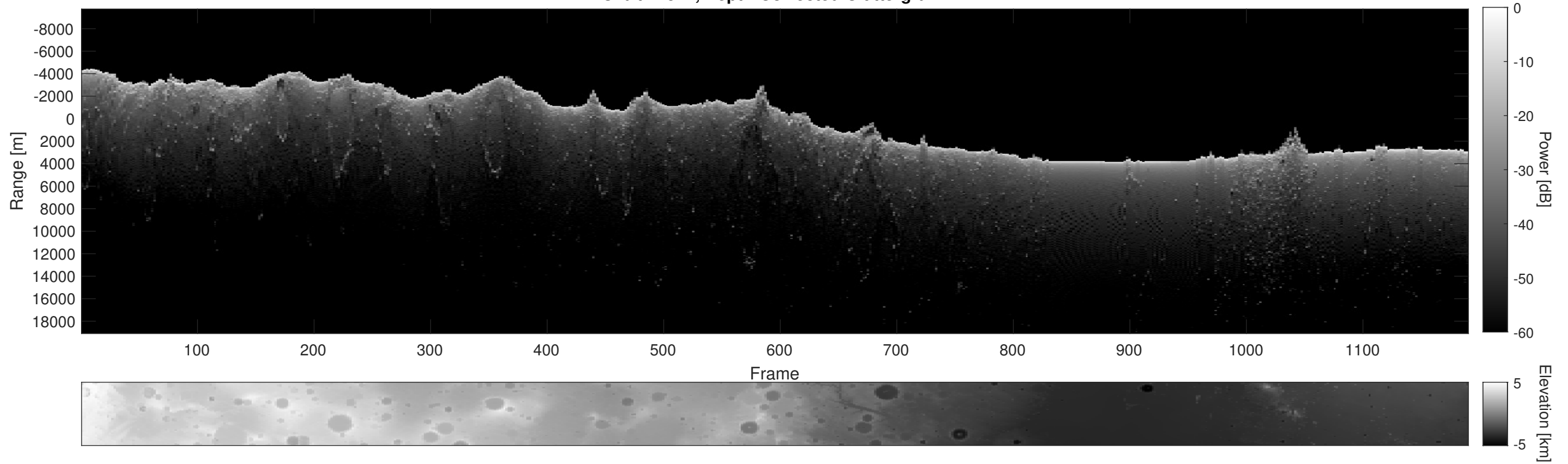
Orbit 12541, Depth-Corrected Cluttergram
