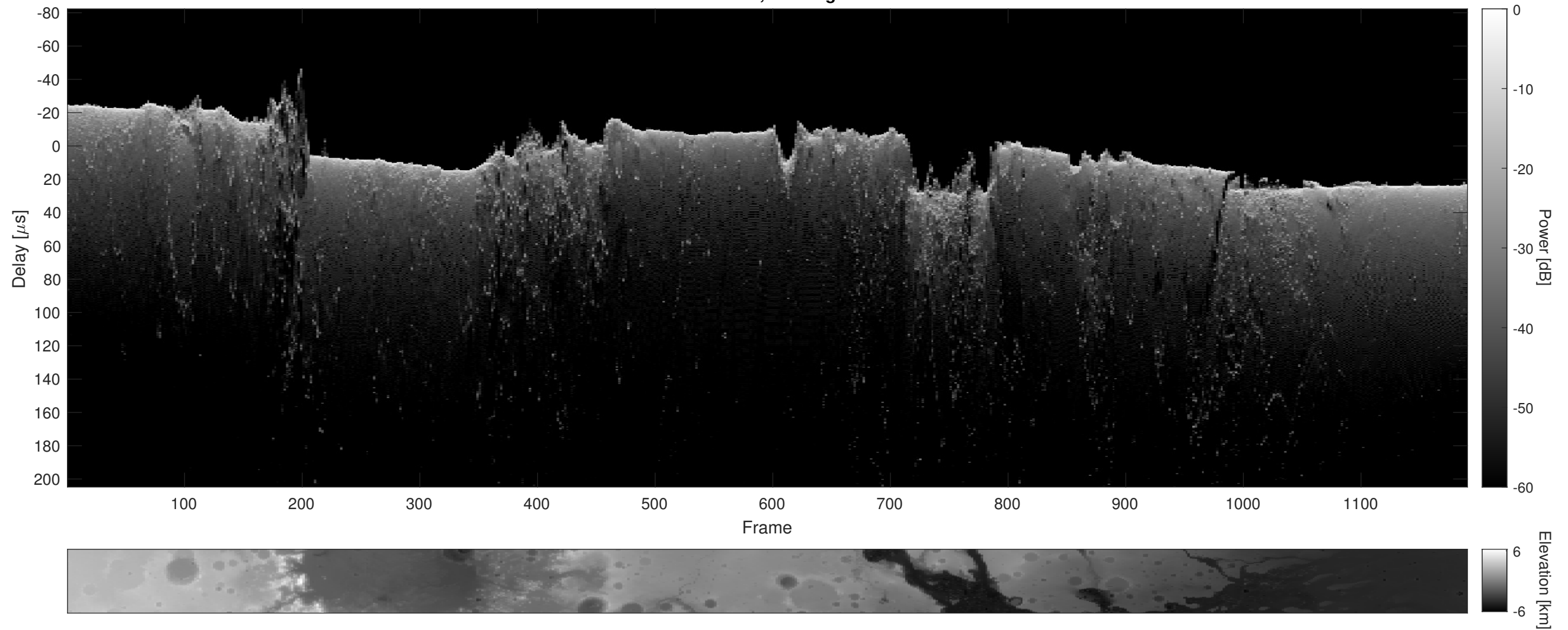
Orbit 12543, Cluttergram
