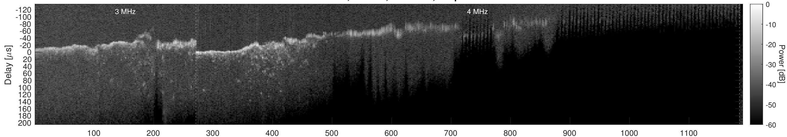
Orbit 12543, Window, Channel 2, Optimized
