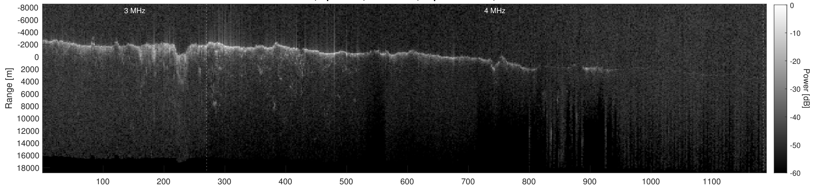
Orbit 12546, Depth-Corrected Cluttergram
