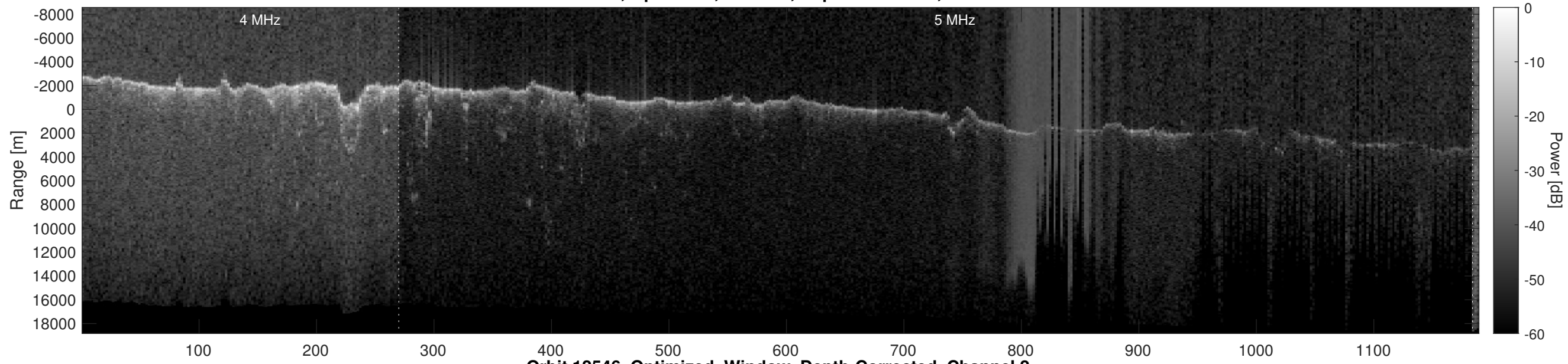
Orbit 12546, Optimized, Window, Depth-Corrected, Channel 2
