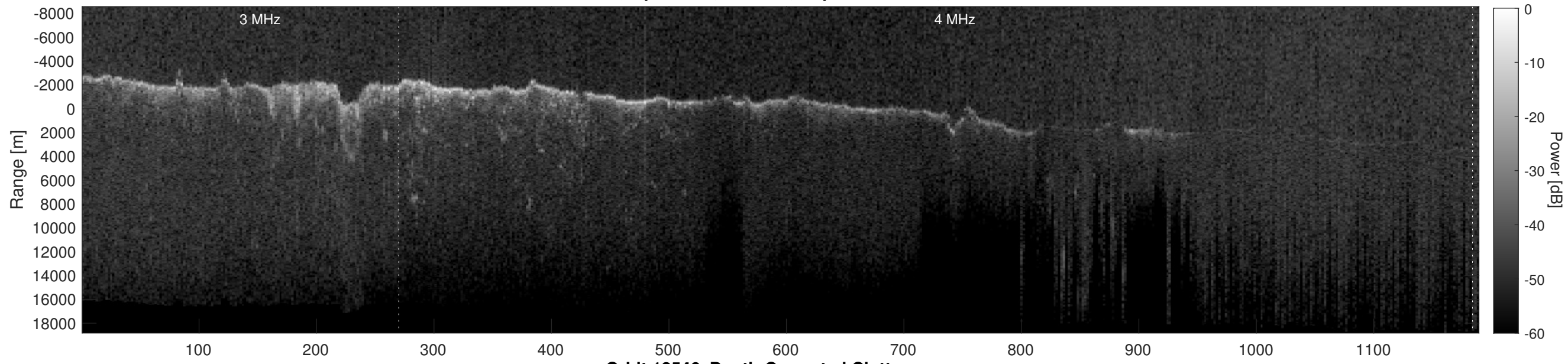
Orbit 12546, Depth-Corrected Cluttergram
