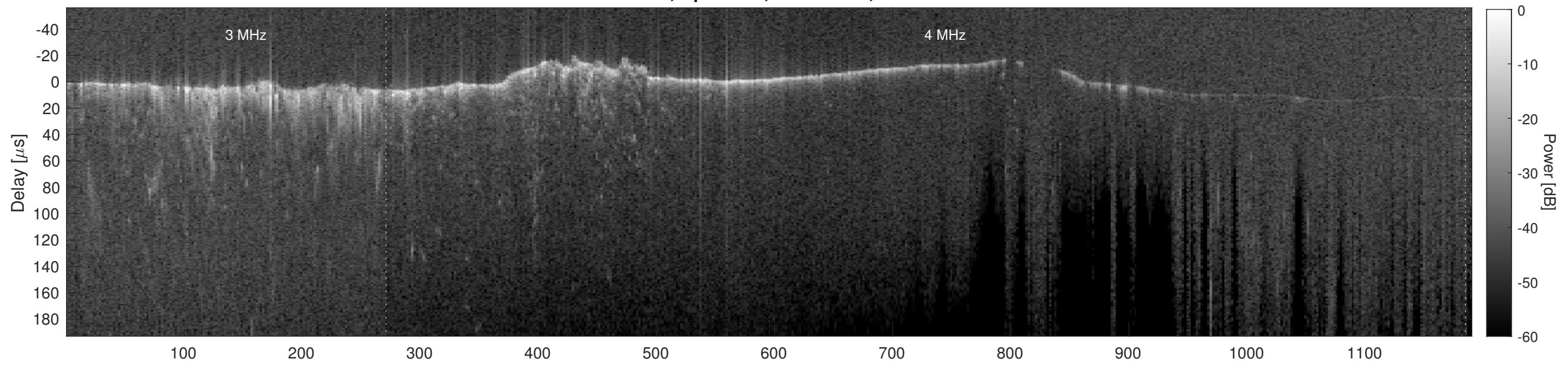
Orbit 12547, Cluttergram
