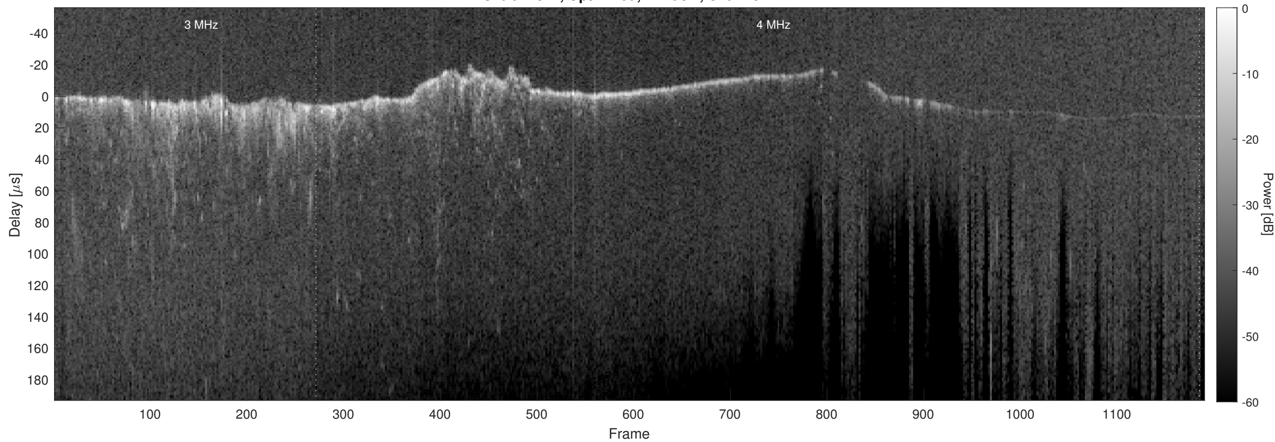
Orbit 12547, Optimized, Window, Channel 2
