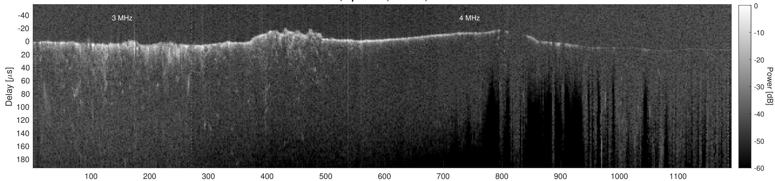
Orbit 12547, Cluttergram
