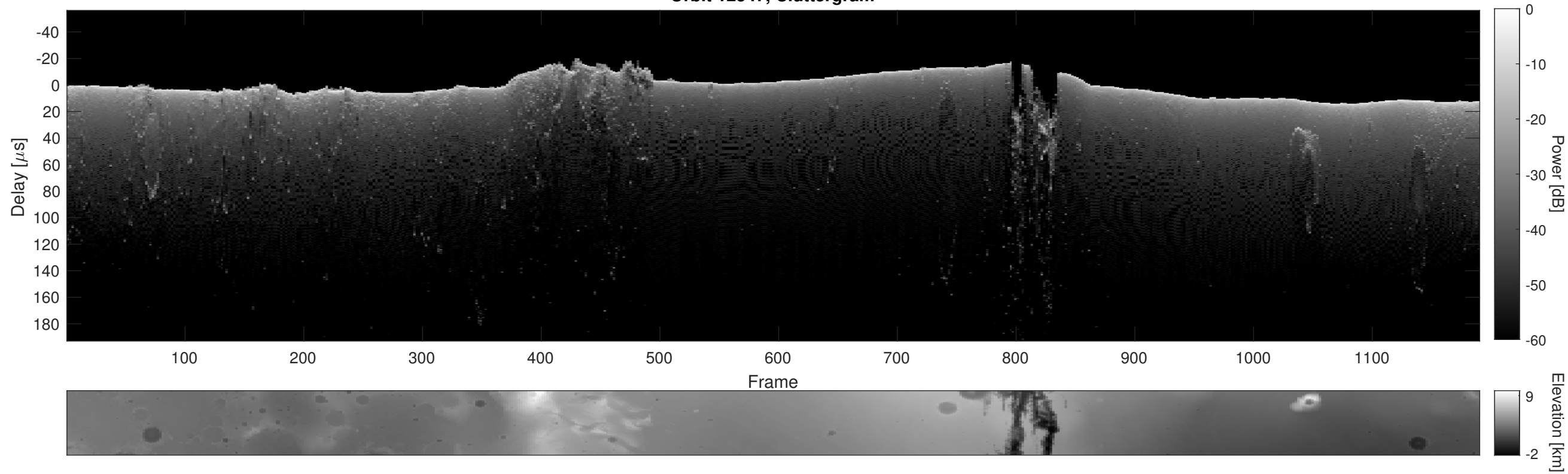
Orbit 12547, Cluttergram
