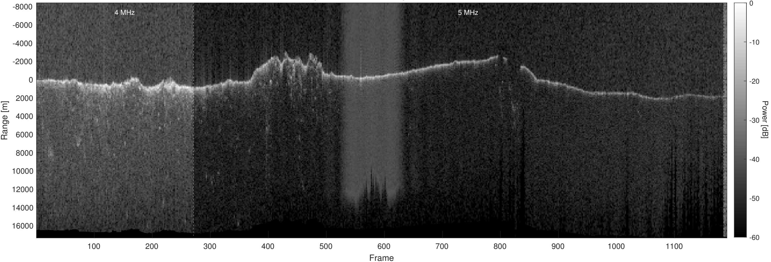
Orbit 12547, Optimized, Window, Depth-Corrected, Channel 2
