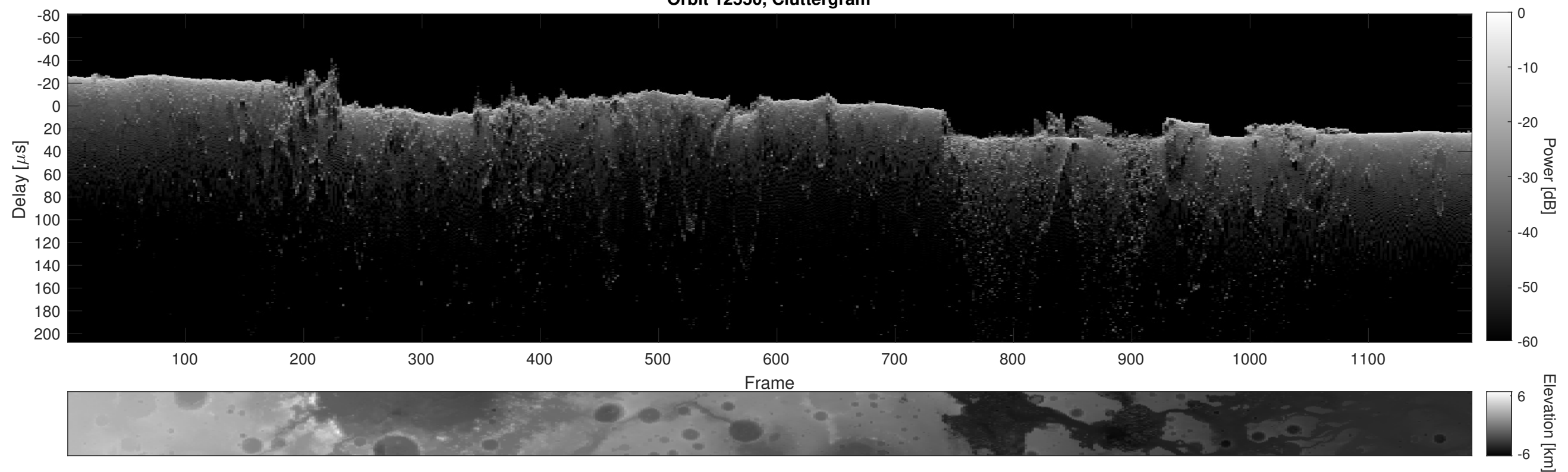
Orbit 12550, Cluttergram
