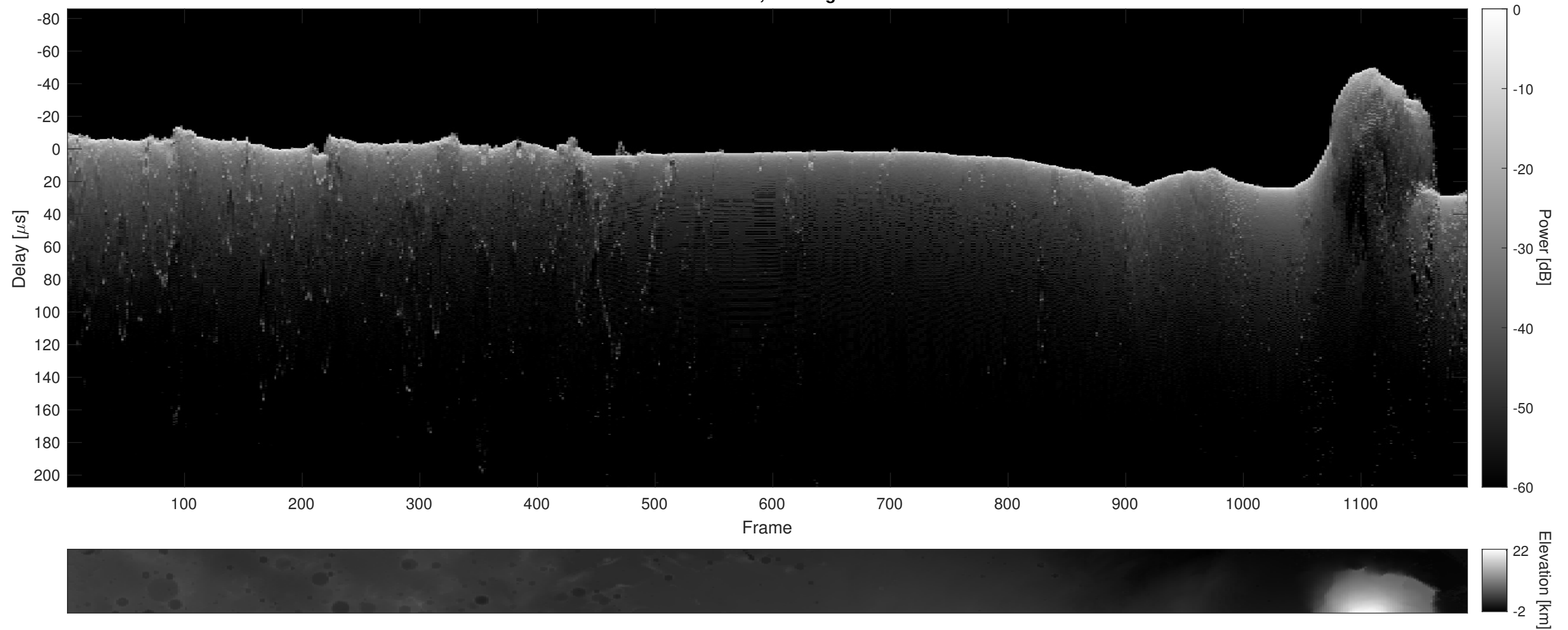
Orbit 12551, Cluttergram
