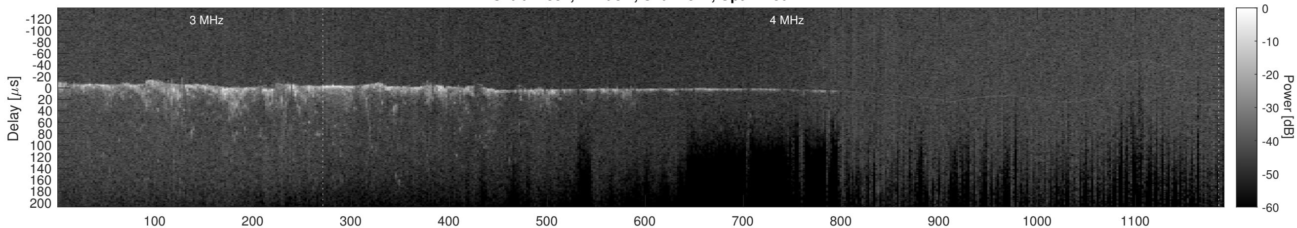
Orbit 12551, Cluttergram
