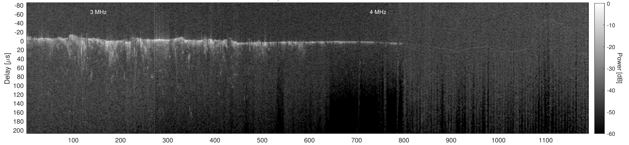
Orbit 12551, Cluttergram
