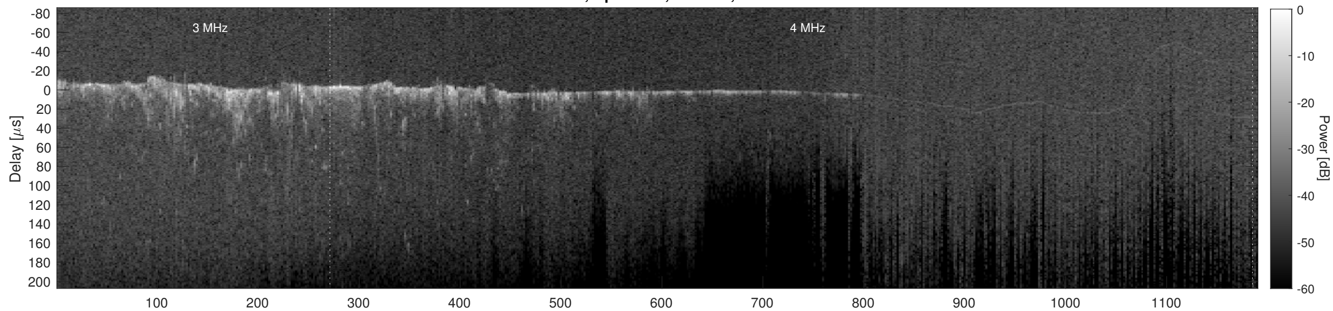
Orbit 12551, Cluttergram
