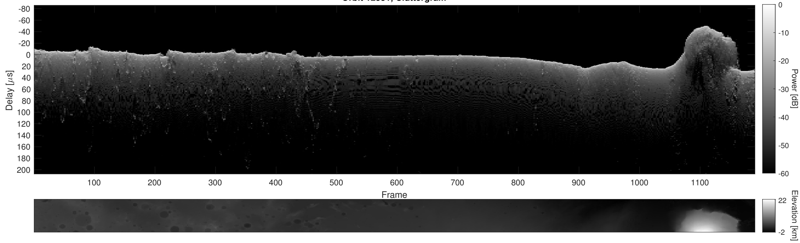
Orbit 12551, Cluttergram
