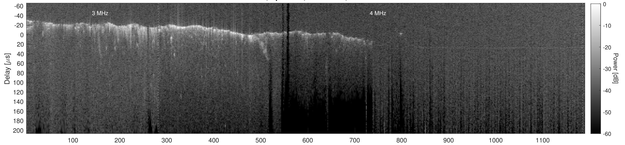
Orbit 12555, Cluttergram
