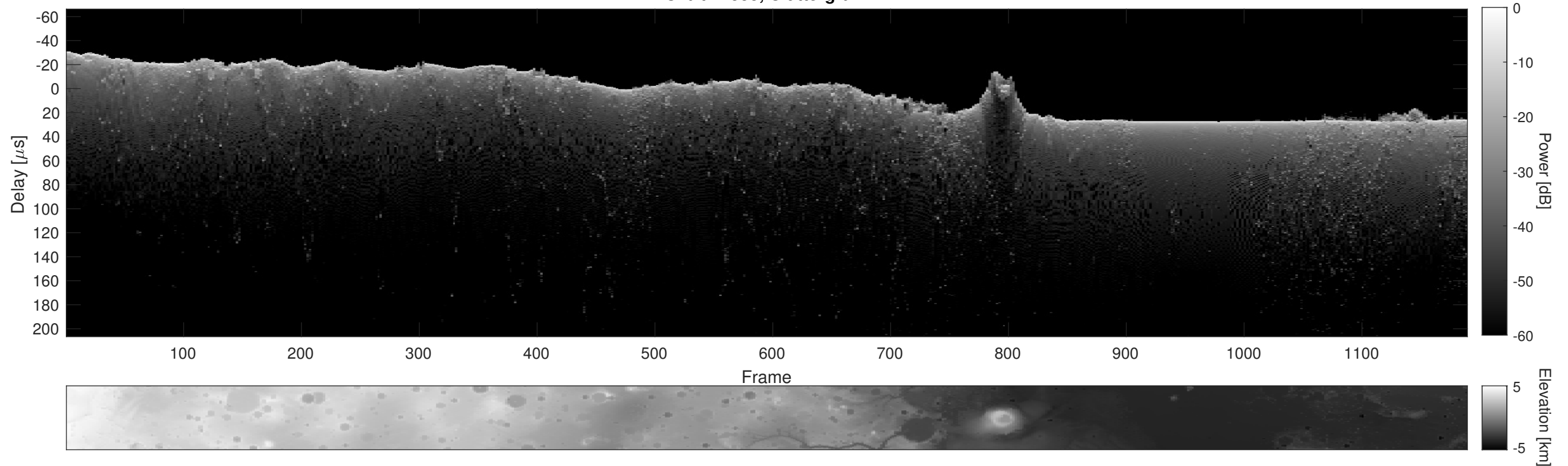
Orbit 12555, Cluttergram
