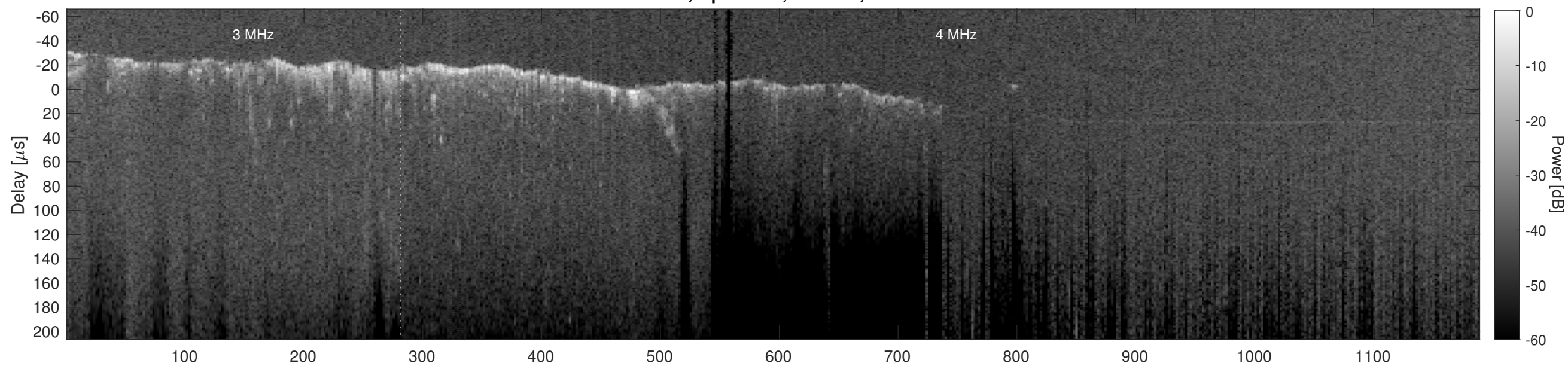
Orbit 12555, Cluttergram
