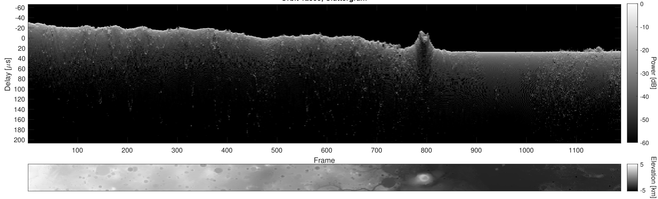
Orbit 12555, Cluttergram
