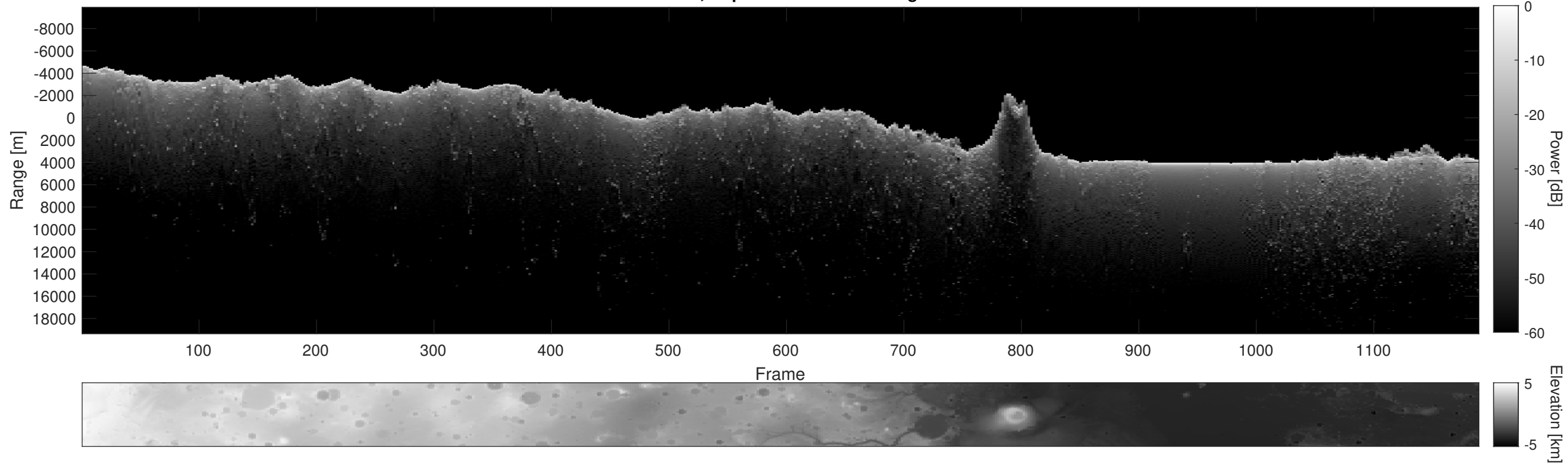
Orbit 12555, Depth-Corrected Cluttergram
