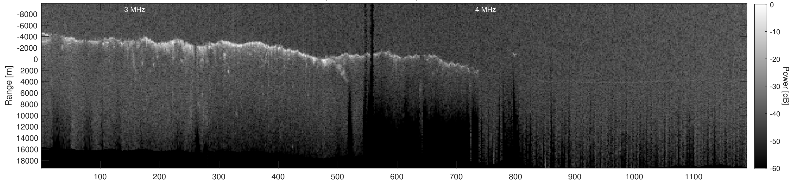
Orbit 12555, Depth-Corrected Cluttergram
