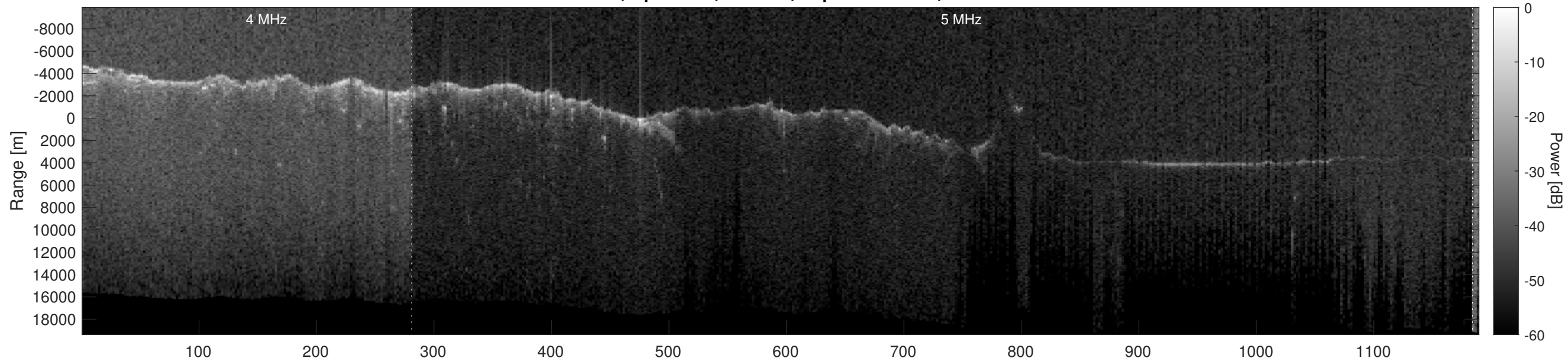
Orbit 12555, Optimized, Window, Depth-Corrected, Channel 2
