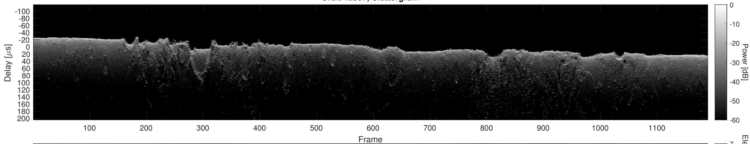
Orbit 12557, Cluttergram
