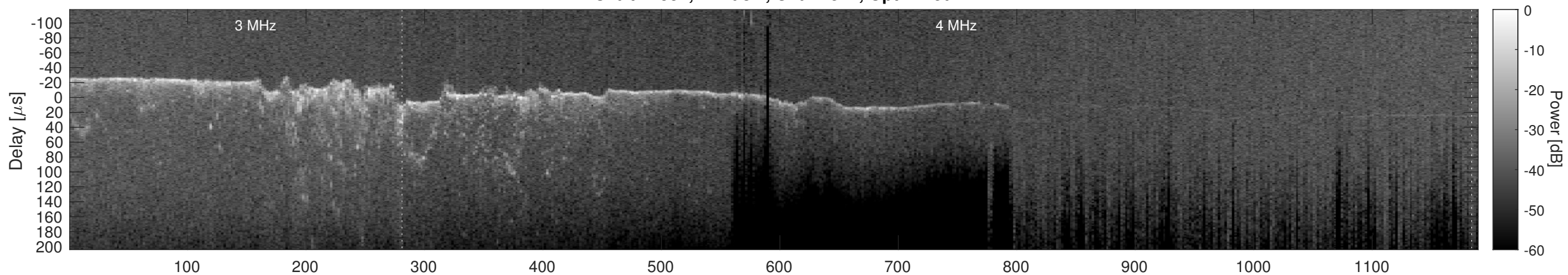
Orbit 12557, Cluttergram
