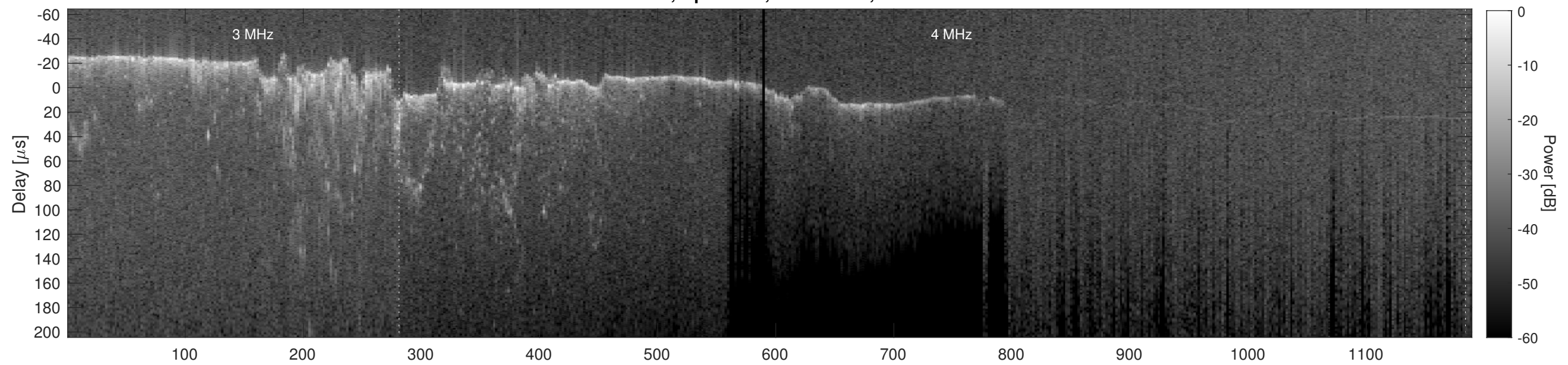
Orbit 12557, Cluttergram
