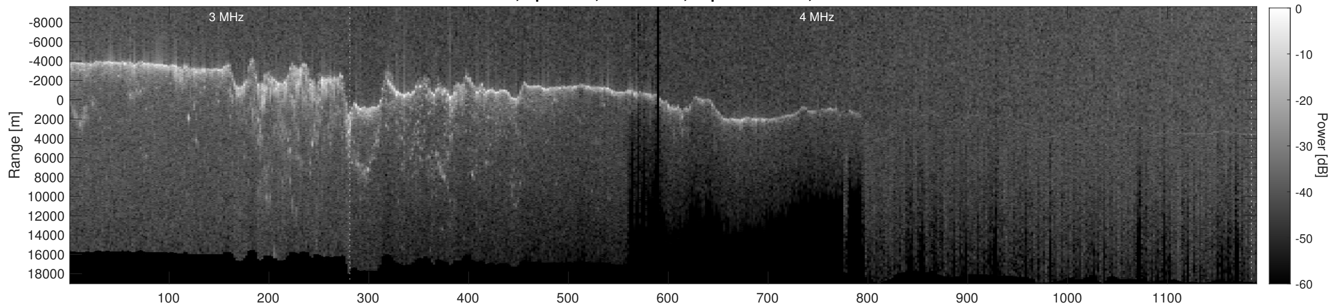
Orbit 12557, Depth-Corrected Cluttergram
