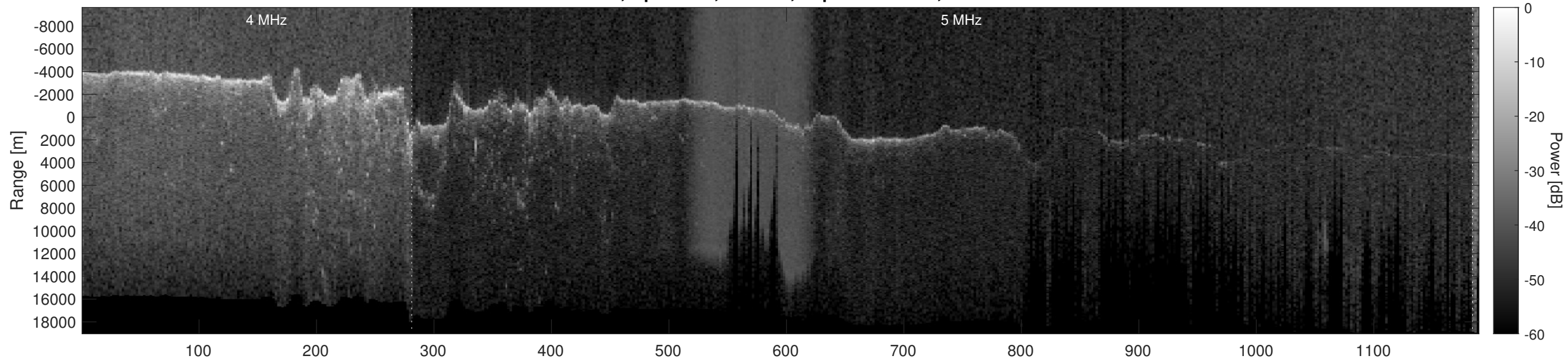
Orbit 12557, Optimized, Window, Depth-Corrected, Channel 2
