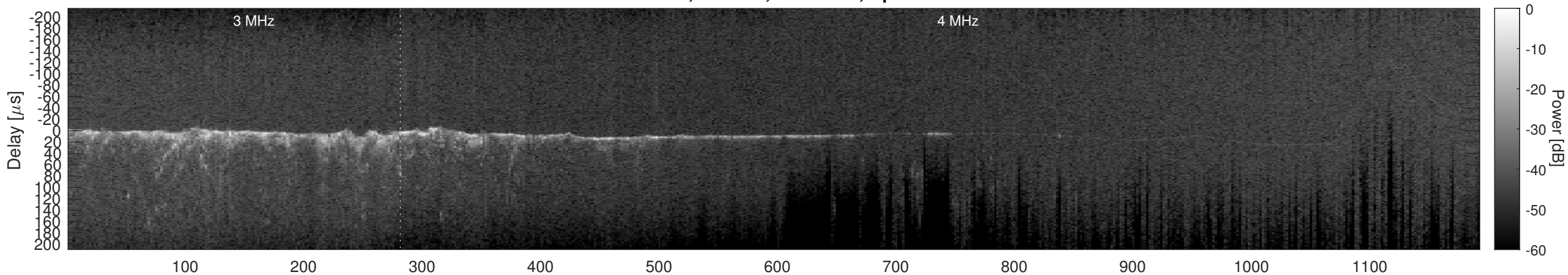
Orbit 12558, Cluttergram
