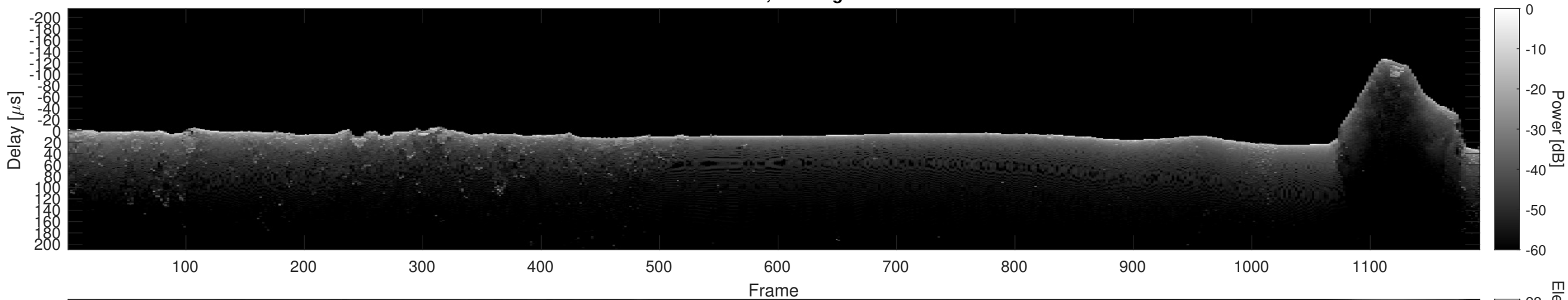
Orbit 12558, Cluttergram
