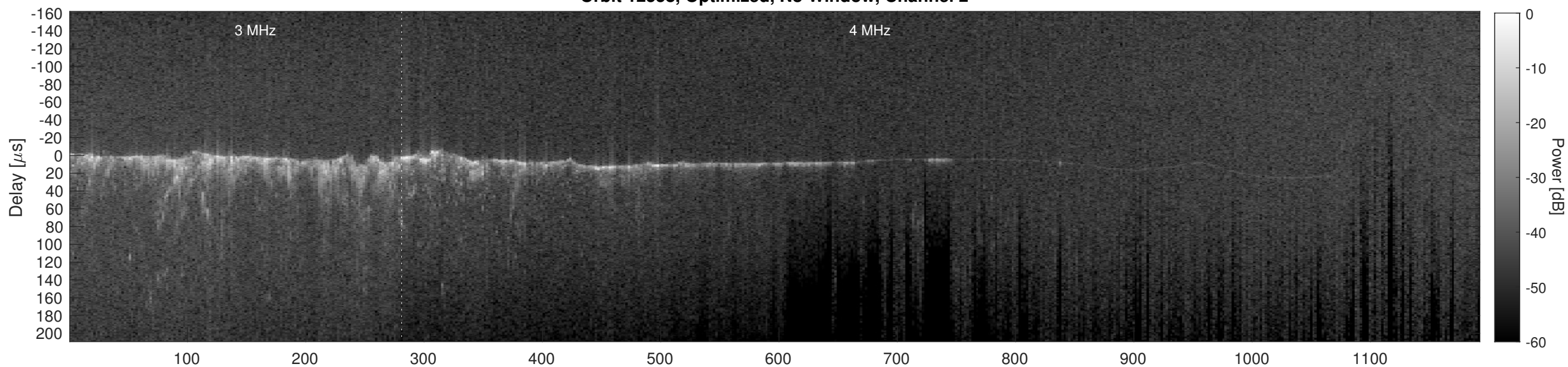
Orbit 12558, Cluttergram
