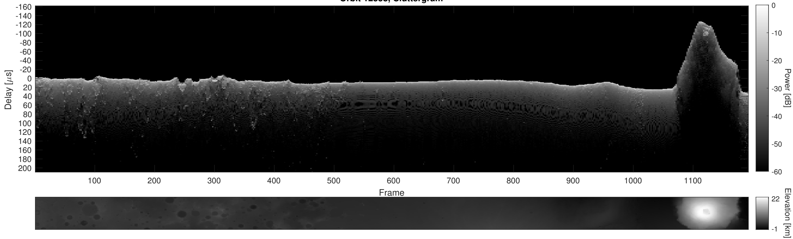
Orbit 12558, Cluttergram
