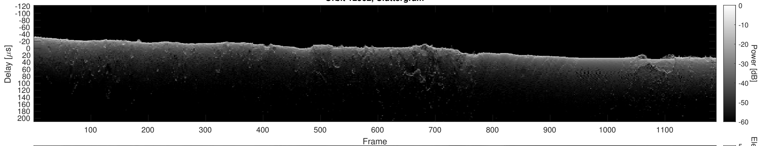
Orbit 12562, Cluttergram
