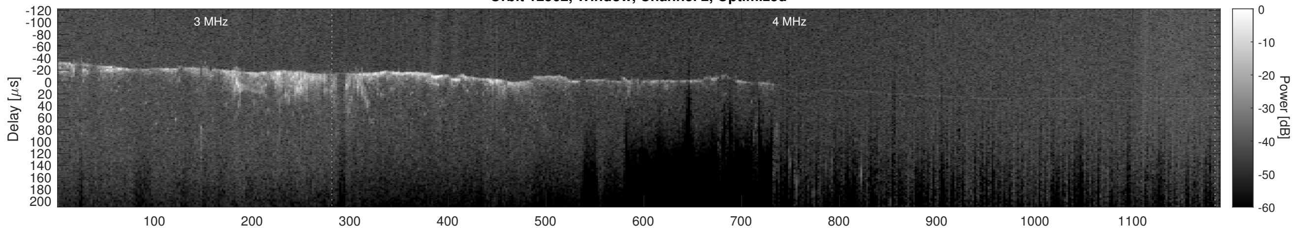
Orbit 12562, Cluttergram
