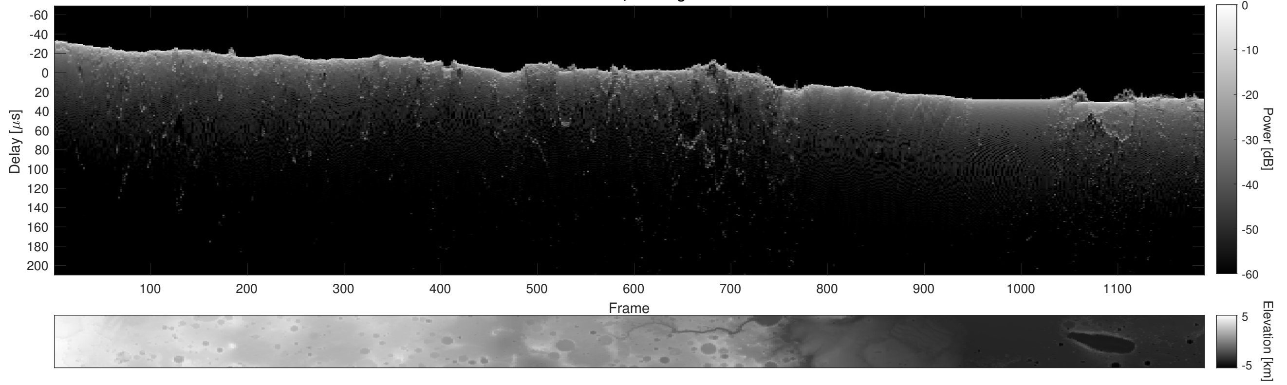
Orbit 12562, Cluttergram
