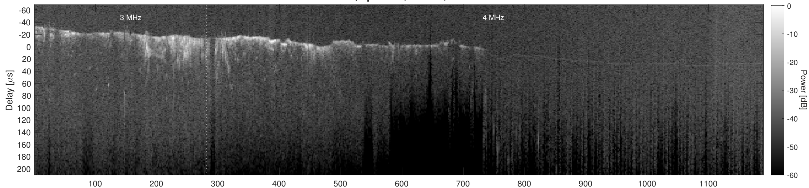
Orbit 12562, Cluttergram
