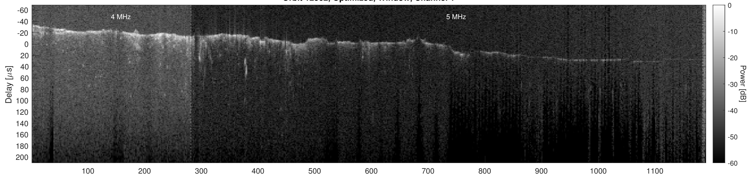
Orbit 12562, Optimized, Window, Channel 2
