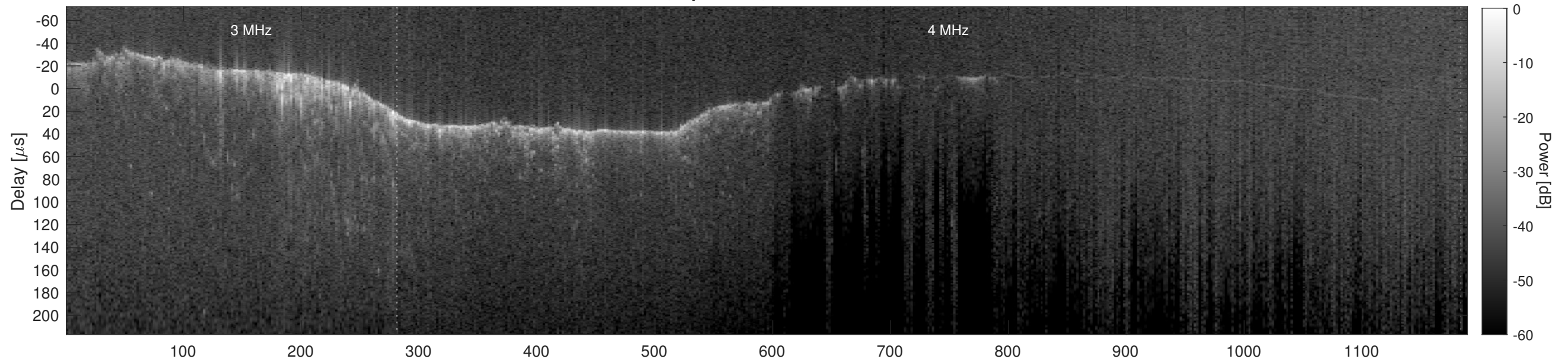
Orbit 12563, Cluttergram
