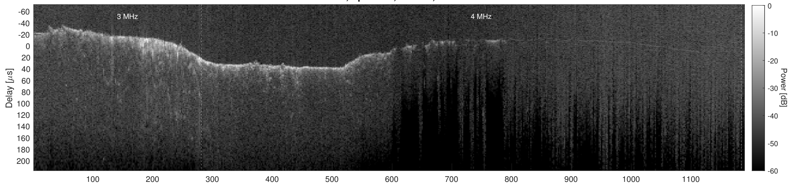
Orbit 12563, Cluttergram
