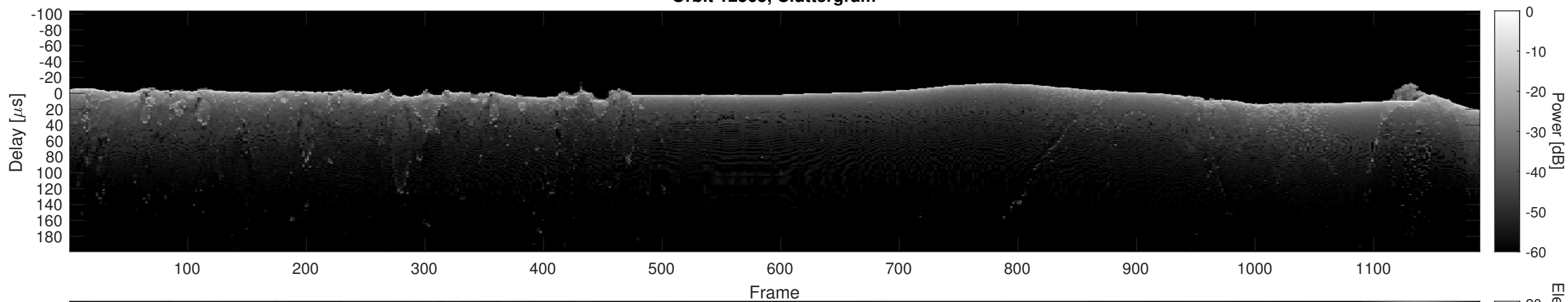
Orbit 12565, Cluttergram
