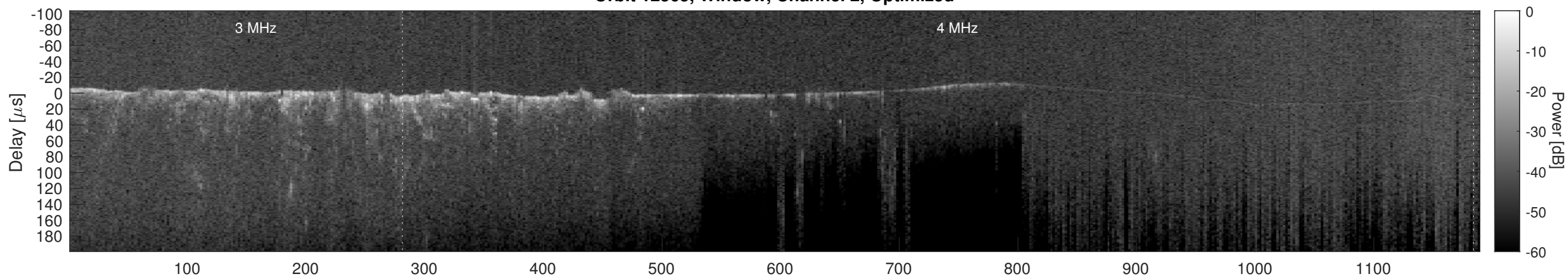
Orbit 12565, Cluttergram
