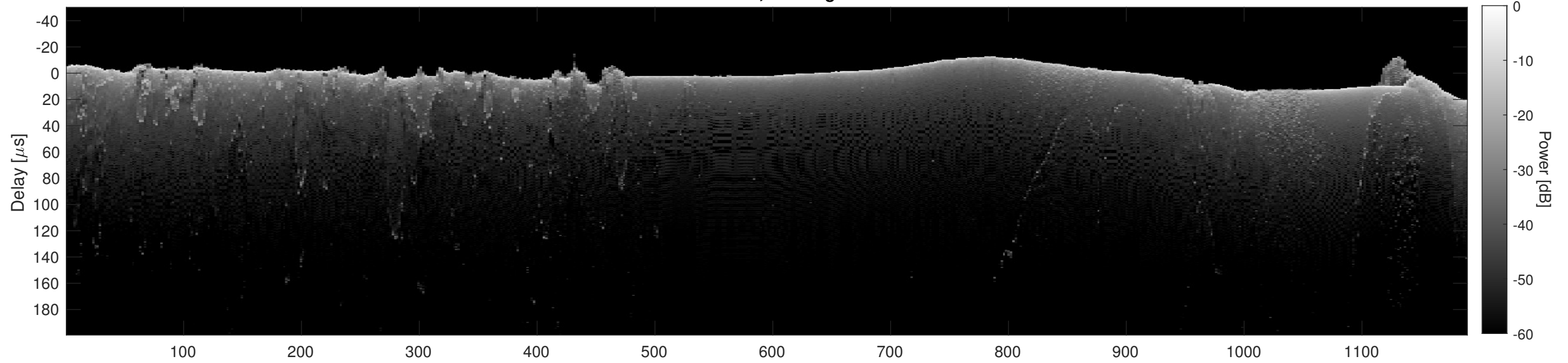
Orbit 12565, Cluttergram
