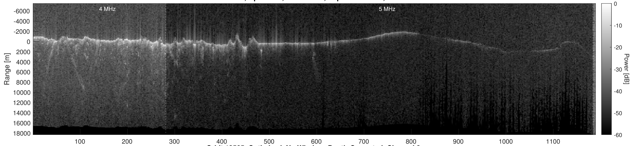
Orbit 12565, Optimized, No Window, Depth-Corrected, Channel 2
