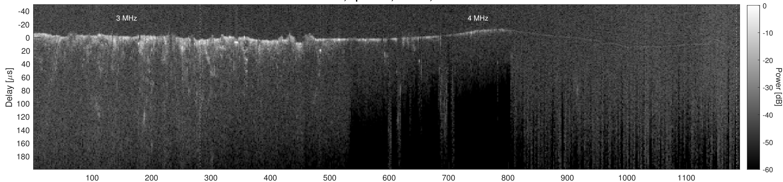
Orbit 12565, Cluttergram
