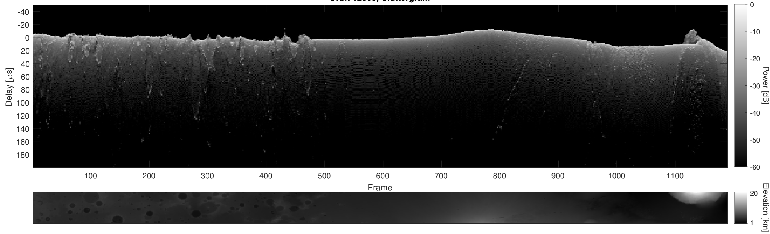
Orbit 12565, Cluttergram
