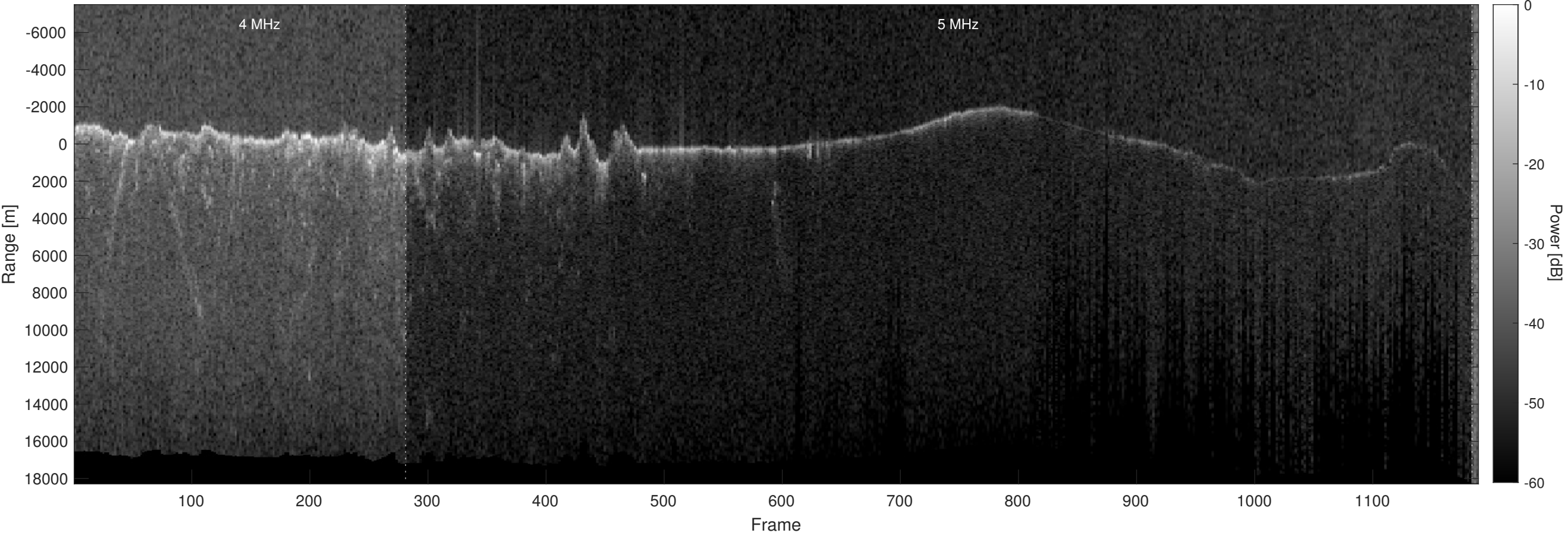
Orbit 12565, Optimized, Window, Depth-Corrected, Channel 2
