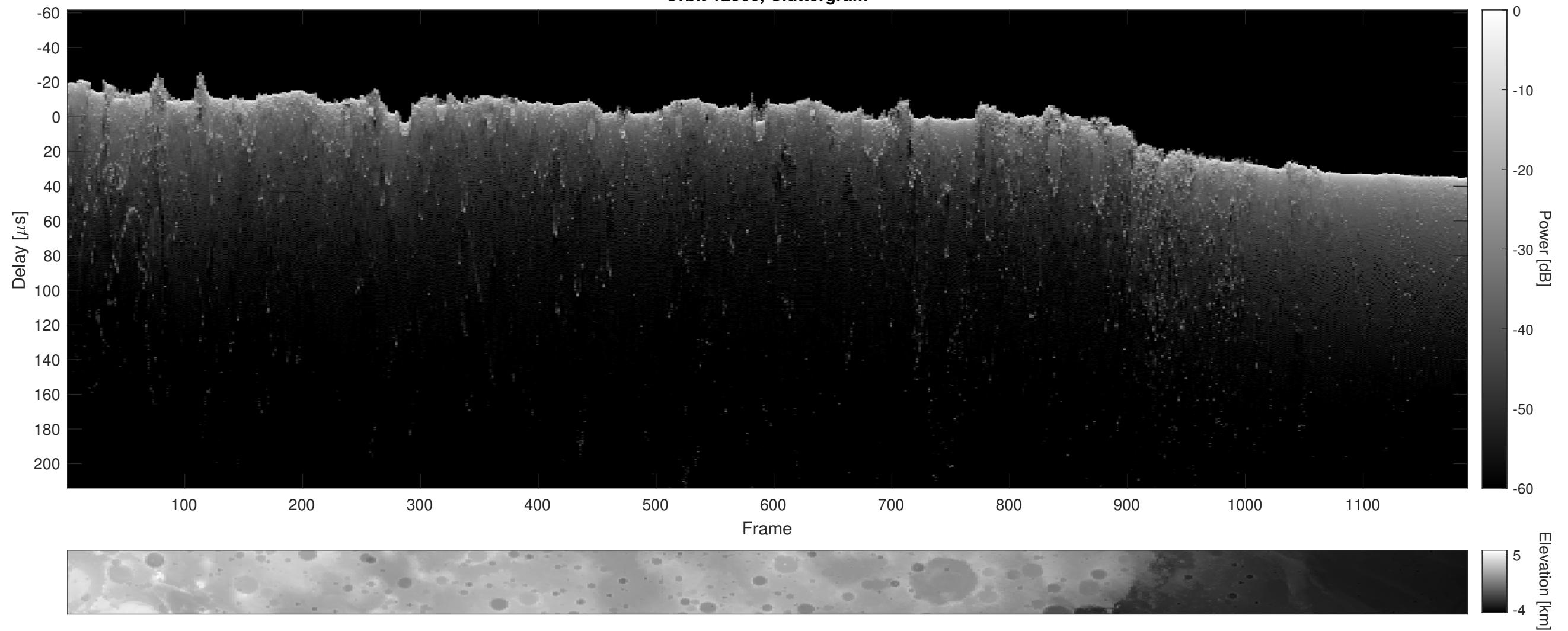
Orbit 12566, Cluttergram
