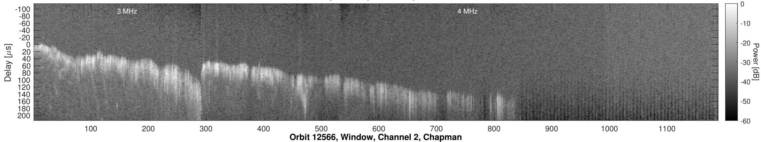
Orbit 12566, Window, Channel 2, Uncorrected
